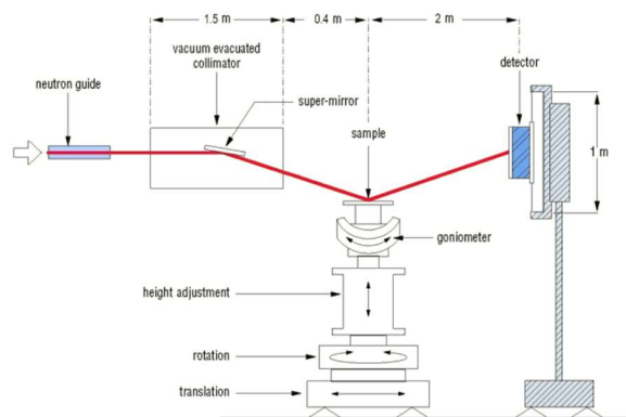
Fig. 1. Scheme of the HERMES reflectometer.
