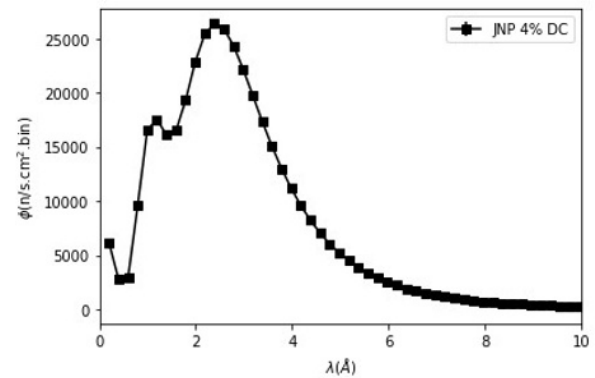
Fig. 3. Simulated source spectra at the JNP at 10 \mu A and 4 % duty-cycle (bin size: 0.2 \text{\AA} ).
